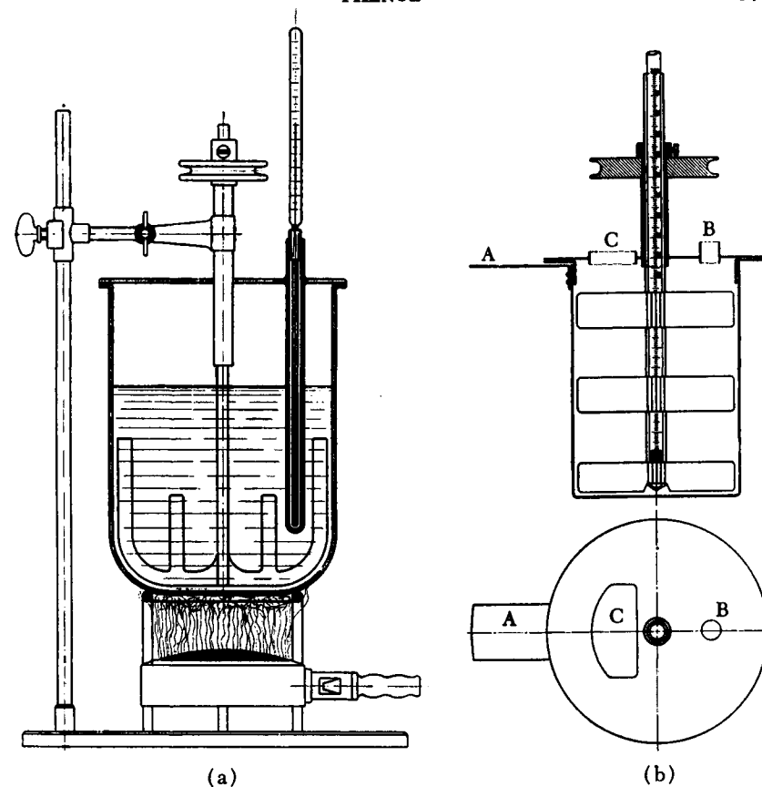
Fig. 14. (a) Fusion kettle for alkali fusions. (b) Fusion kettle with central thermometer tube: A, handle, attached by rivets, for securing the kettle; B, opening for introducing gases; C, filling port.
