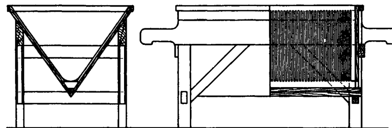
Fig. 27. Portable filter for coarsely crystalline precipitates.
