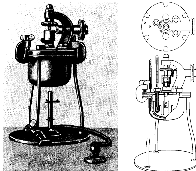
Fig. 36. Iron fusion kettle with copper oil bath for use in primuline, indigo, and alkali fusions, etc. Capacity, about 450 cc.
