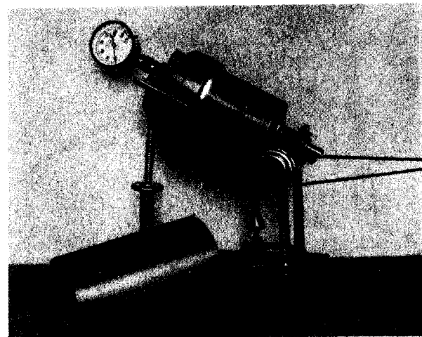
Figure 49. Rotating wrought iron autoclave with worm gear drive: weight, 11 kg; capacity, 400 cc.; working pressure, 100 atm.
