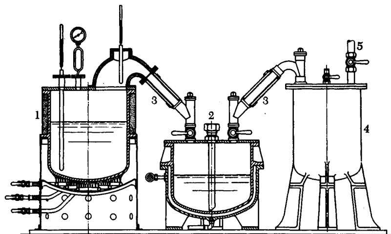
Fig. 40. Vacuum distillation equipment for substances which solidify easily (naphthols, phenylenediamine, etc.). The apparatus for large quantities (1000–3000 kg.) is equipped with a stirring mechanism to prevent charring. 1, distillation vessel; 2, receiver with steam or water jacket; 3, steam heated tubes to prevent solidification; 4, trap to collect water and sublimate; 5, line to pump.
