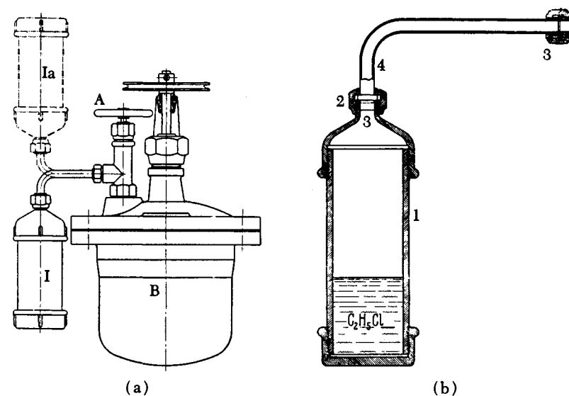
Fig. 25. (a) Method of introducing alkyl chloride into a laboratory autoclave. (b) Auxiliary cylinder (gas pipe) for handling alkyl chlorides.
