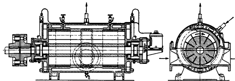
Fig. 39. Rotary compressor and vacuum pump.
