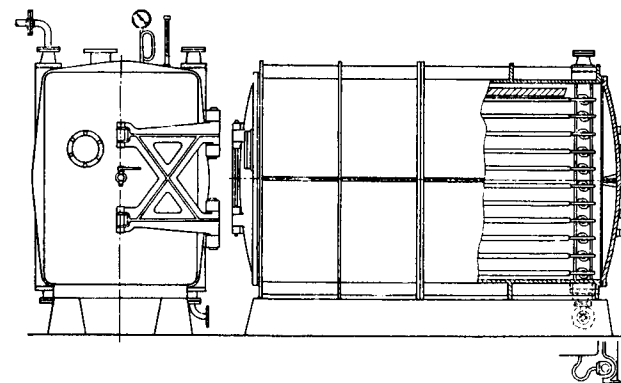
Fig. 52. Vacuum drying oven for dyes.
