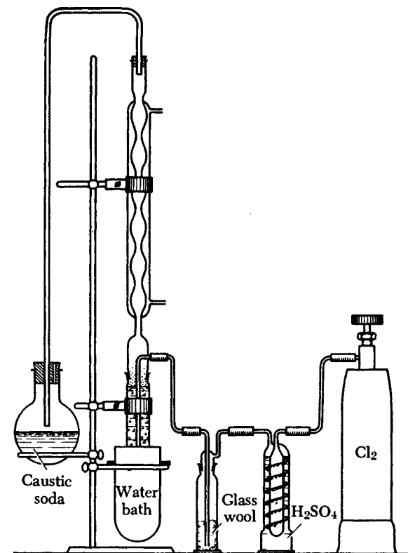
Fig. 5. Laboratory chlorination apparatus.
