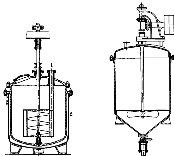
Fig. 8. Nitration kettle with auger-type stirrer, equipped for external and internal cooling: (1) water inlet tube for internal cooling; (2) heating and cooling jacket.
