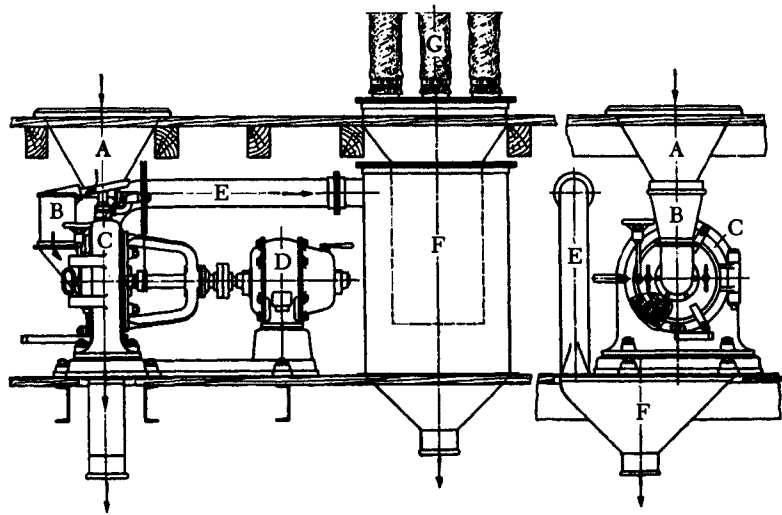
Fig. 54. Disintegrator for dyes: (A) feed hopper; (B) oscillating feed with magnetic screening device; (C) disintegrator; (D) motor; (E) dust pipe; (F) dust chamber; (G) filter bags.
