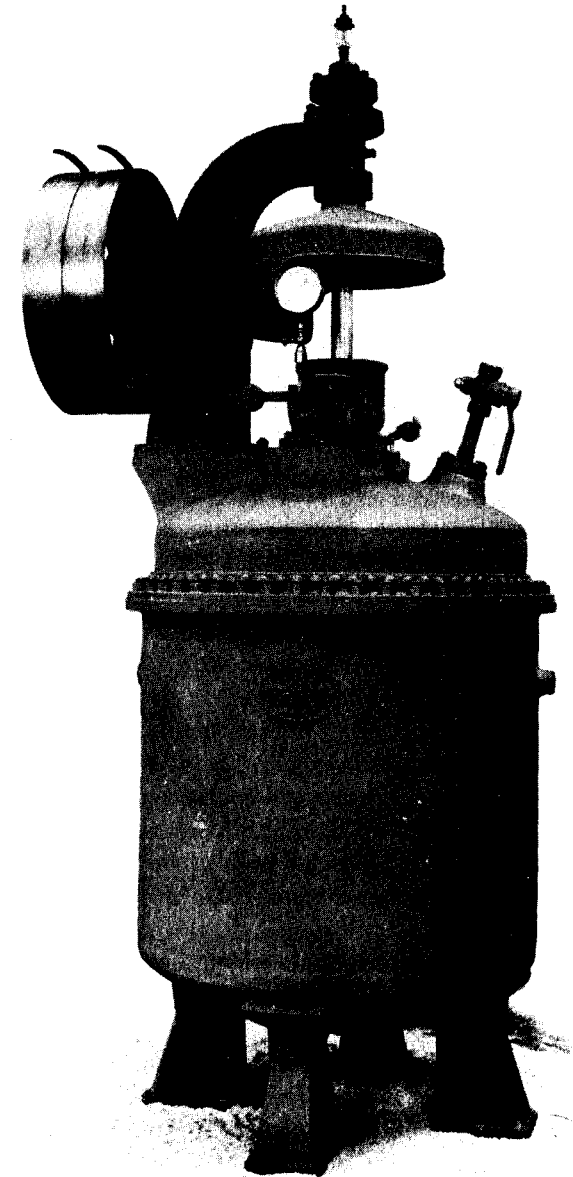
Fig. 44. Cast iron works autoclave with steam heating. Capacity is 1400 liters; maximum pressure, 25 atm. The stirrer mount is high so that the stuffing box is easily accessible. Samples can be removed through the cock seen at the upper right.
