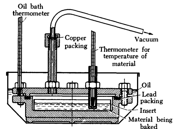
Fig. 30. Vacuum baking apparatus.
