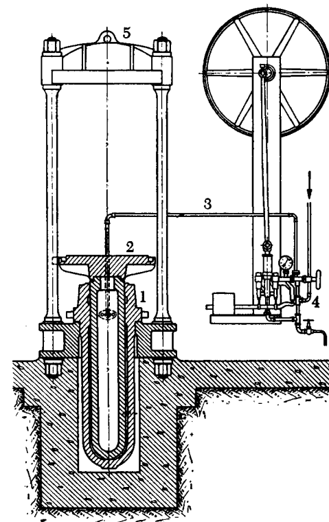
Fig. 12. Hydraulic press with automatic cut-out on pump: (1) cast steel cylinder; (2) press table; (3) inlet tube for pressure fluid (water) (250 atm.); (4) pump which cuts out at 250 atm. (the pressure can be varied by moving the weight; one pump easily serve 4 to 6 presses); (5) cast steel head-piece.
