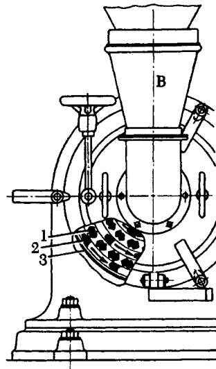
Fig. 53. Sketch of the "Perplex" disintegrator: (B) feed; (1) stationary hammers; (2) rotating hammers, 1200-2000 r.p.m.; (3) sieve.
