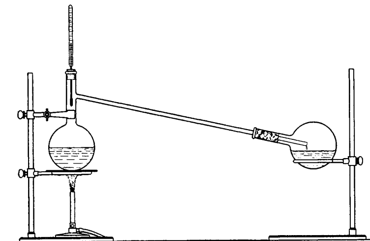
Fig. 7. Distillation apparatus for high-boiling liquids.
