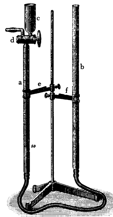
Fig. 10. The Lunge nitrometer.
