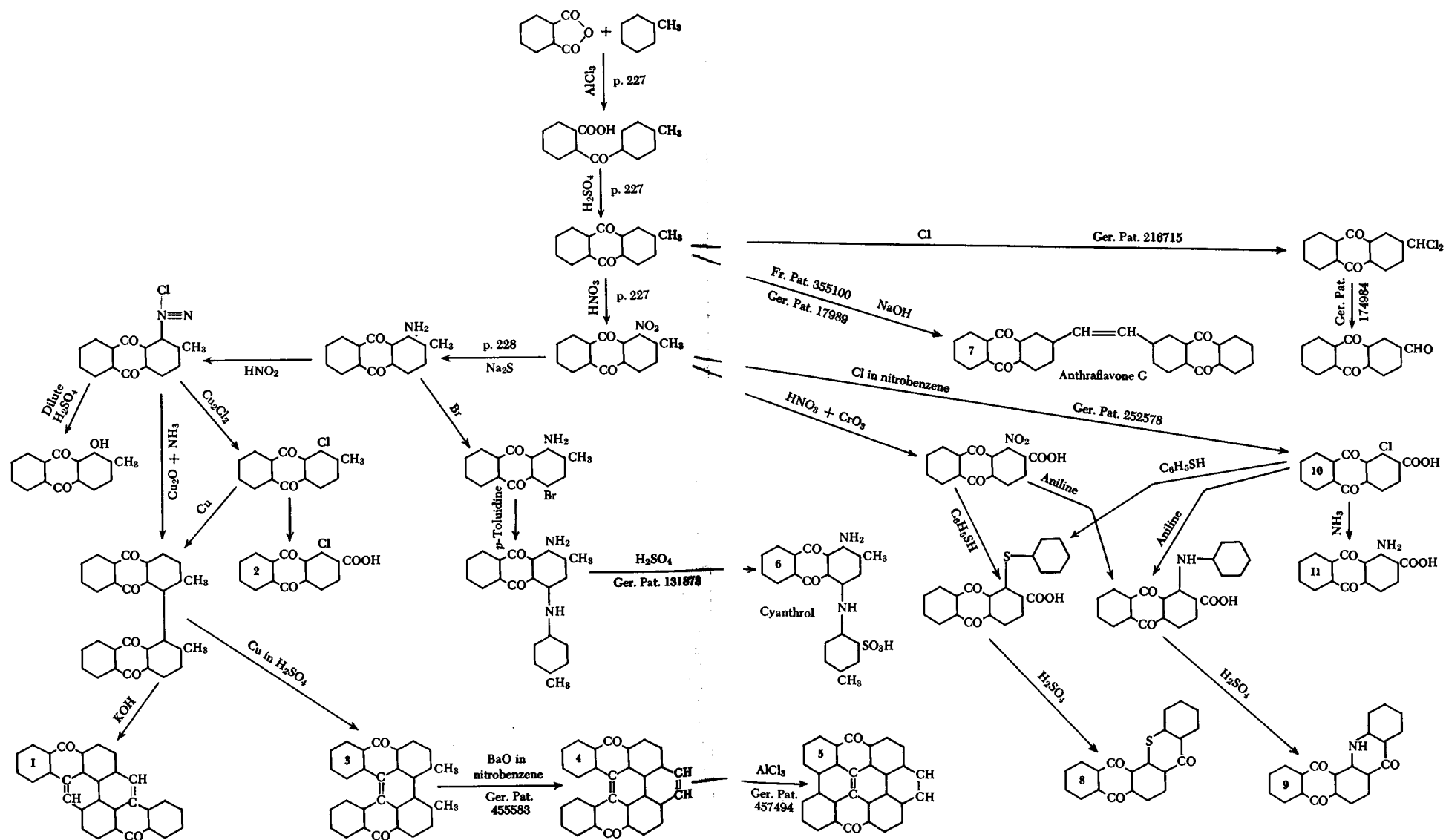
Indanthrene golden orange G
