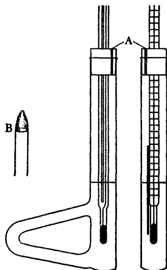
Fig. 3. Thiele melting point apparatus: A, groove for pressure equalization; B, flame.
