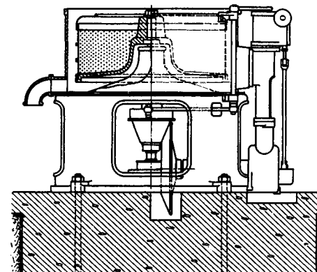
Fig. 33. Centrifuge with bottom discharge.
