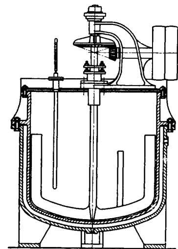
Fig. 31. Sulfonation and nitration kettle with steam jacket (double wall).
