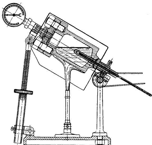
Fig. 50. Cross section through the rotating autoclave.
