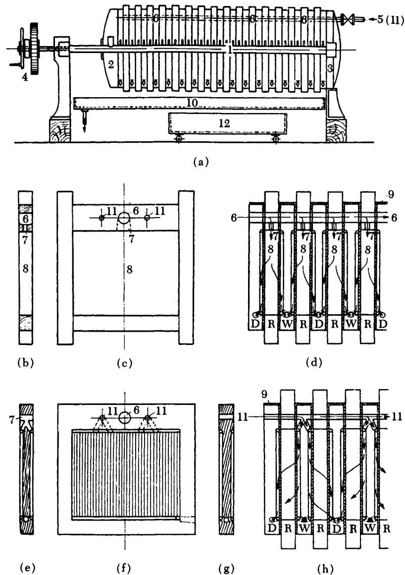
Fig. 42. Filter press: (a) assembled press; (b, c) filter frame, R; (d) filtering; (e, f) wash plates, W; (g) filter plates, D; (h) washing.
