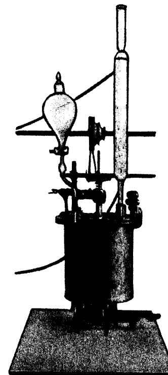
Fig. 11. Closed, coppered reduction vessel fitted with stirrer, dropping funnel, and reflux condenser, for use with substances volatile with steam.
