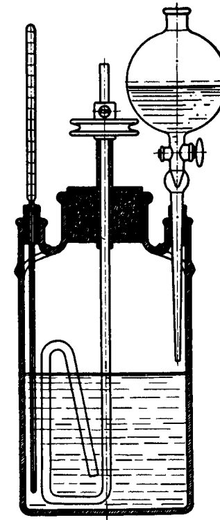
Fig. 20. Autogenously welded sulfonation vessel, especially for use with oleum.
