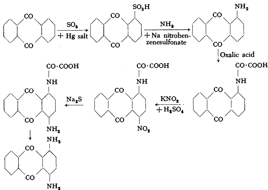
(a) Anthraquinone-1-sulfonic Acid
