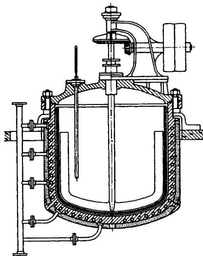
Fig. 34. Kettle heated with steam or hot water (Frederking).
