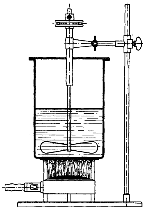
Fig. 17. Apparatus with propeller stirrer for Béchamp-Brimmeyr reductions.
