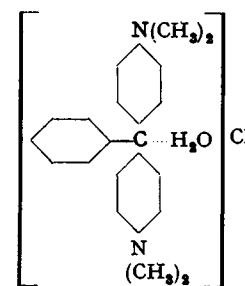
(a) Leuco Malachite Green
