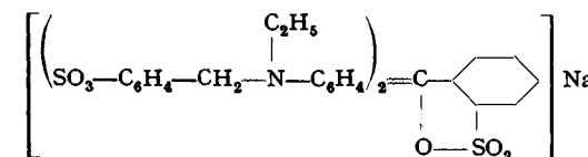
Erioglaucine A from ethylbenzylanilinesulfonic acid and o -sulfo benzaldehyde
