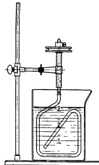
Fig. 32. Graduated vessel for coupling reactions.
